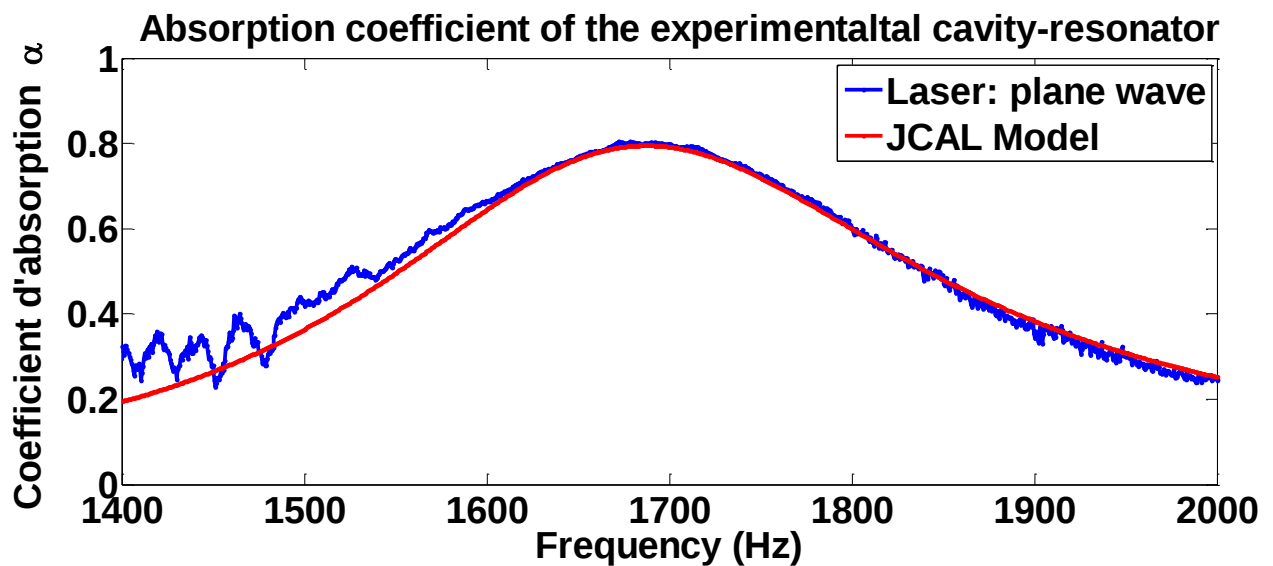
Figure 2: Absorption Coefficient of the quarter-wave resonator cavity (geometry 1)
