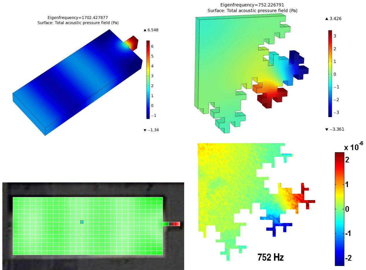
Figure 1 : Acoustic localized modes : top) Numerical results, bottom) Experimental results using laser vibrometer
